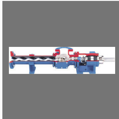
Single Screw Pump/ Progressive Cavity Pump
