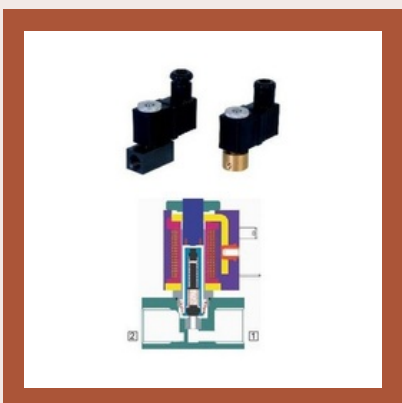
Rotex 2 Port Direct Acting Normally Closed Solenoid Valve(EMS)
